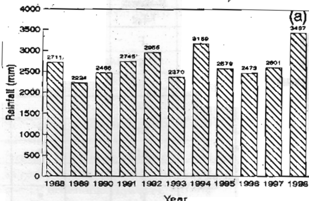
Fig. 1 (a) Cumulated annual rainfall from 1988 to 1998 at Peechi
