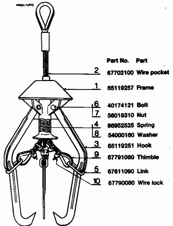
Fig. 2. Skidding Grapple
